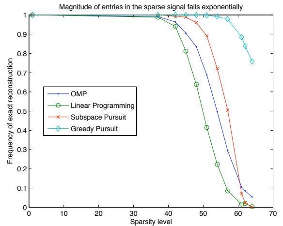
(b) Magnitudes of non-zero entries of \mathbf{x} decay exponentially.
