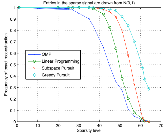
(a) Non-zero entries of \mathbf{x} are distributed \mathcal{N}(0, 1) .
